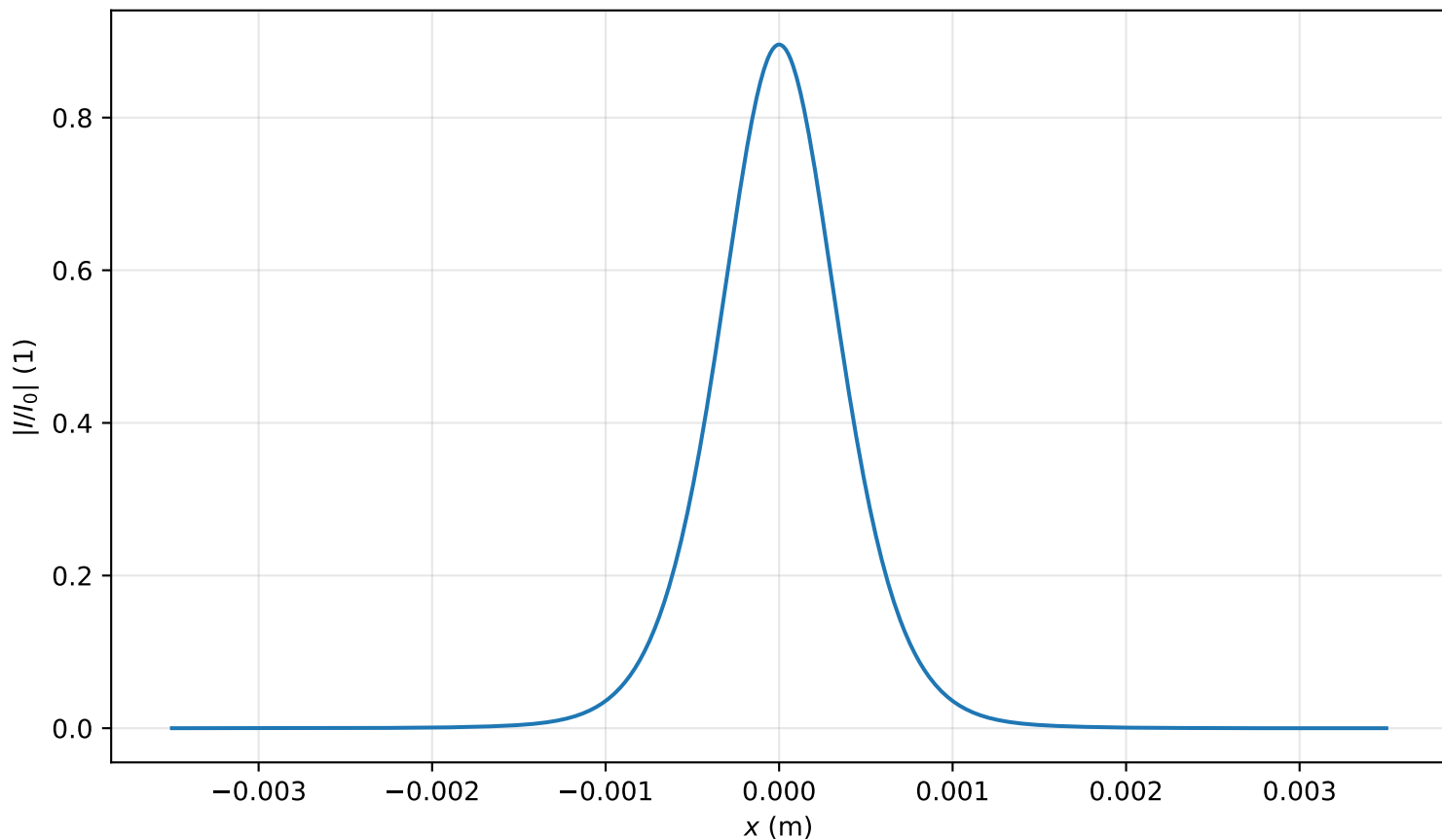
Intensity profile I(x, y = 0, z = 2.786m)/I_0 , P_{in}=0.7P_{cr} , artificial time
